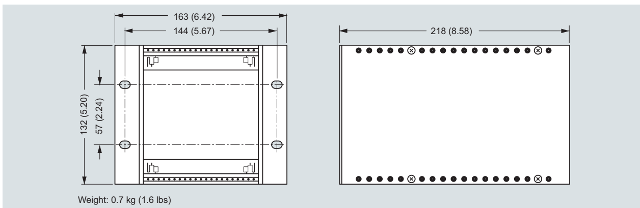
Transmitter back of panel
