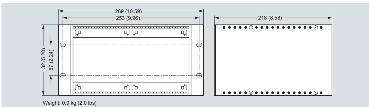
Transmitter back of panel, 42 TE
