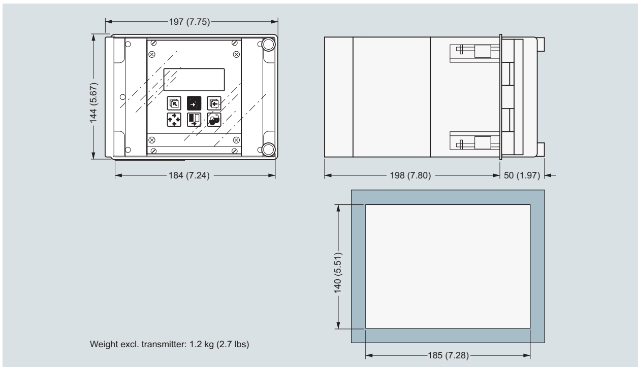
Transmitter 19" front of panel
