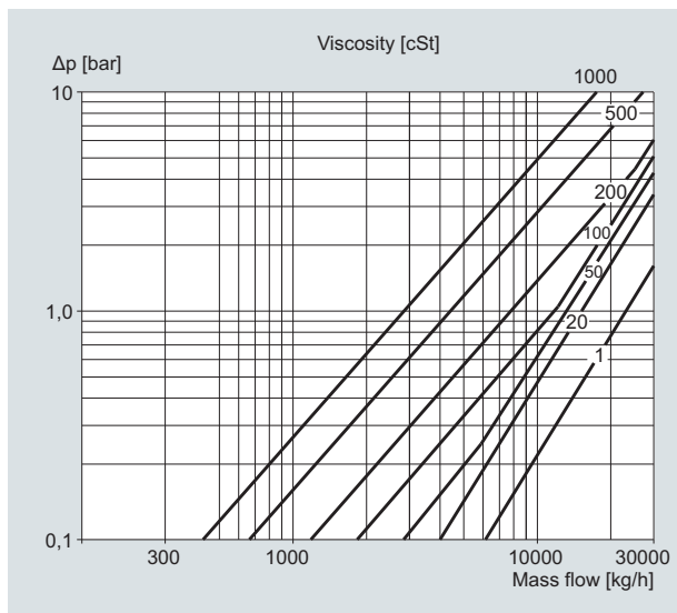
MASS 2100 DI 25 (1"), pressure drop for density = 1000 kg/m 3
