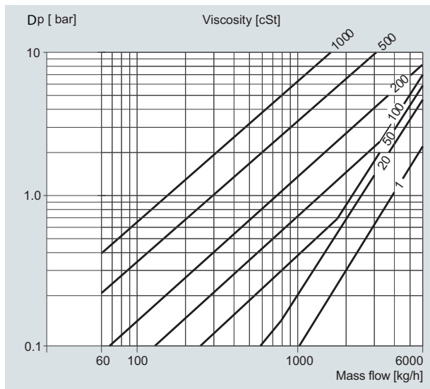
MASS 2100 DI 15 (1/2"), pressure drop for density = 1000 kg/m 3
