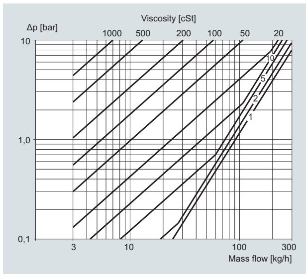
MASS 2100 DI 3 (1/8"), pressure drop for density = 1000 kg/m 3
