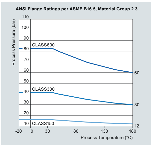
ASME flanges B16.5 stainless steel
