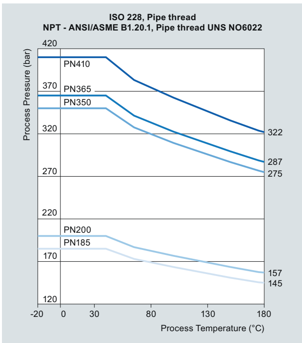
ISO 218 and NPT flanges stainless steel (PN 185 ... PN 410)
