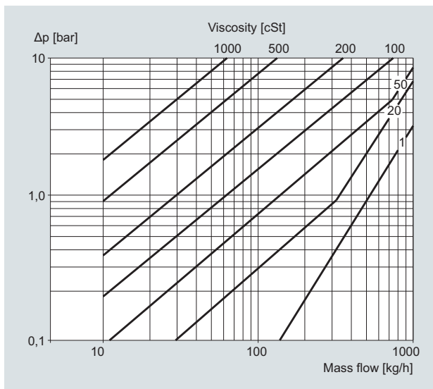
MASS 2100 DI 6 (1/4"), pressure drop for density = 1000 kg/m 3
